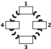
Default FM carrier/modulator relationship between the 4 oscillators on the front panel
